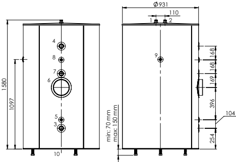
LCT INOX 750
