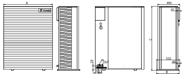
AHP 70-15 AHP 70-18
